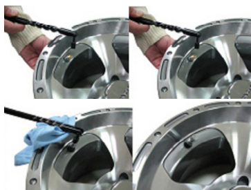
Tyre valve stem inserter
